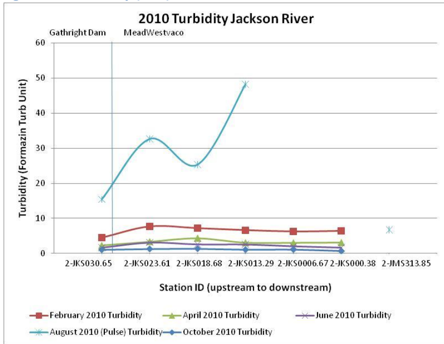
Figure 20. Turbidity (FTU) 2010.
