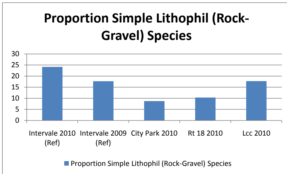
Figure 57. Proportion of simple lithophil (rock-gravel) species collected at each Jackson River sampling site.
