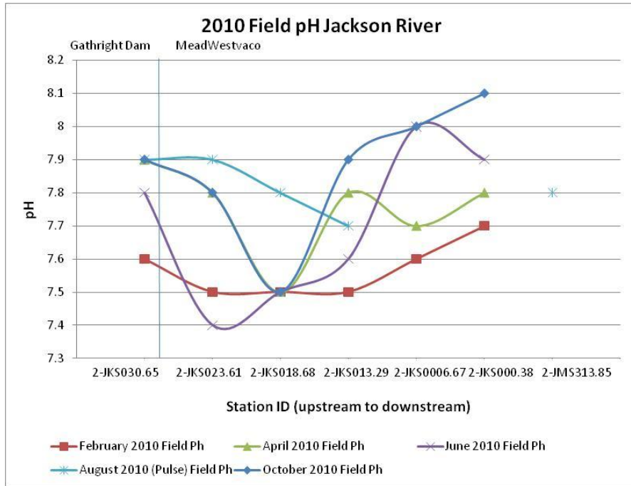
Figure 3. pH 2010.
