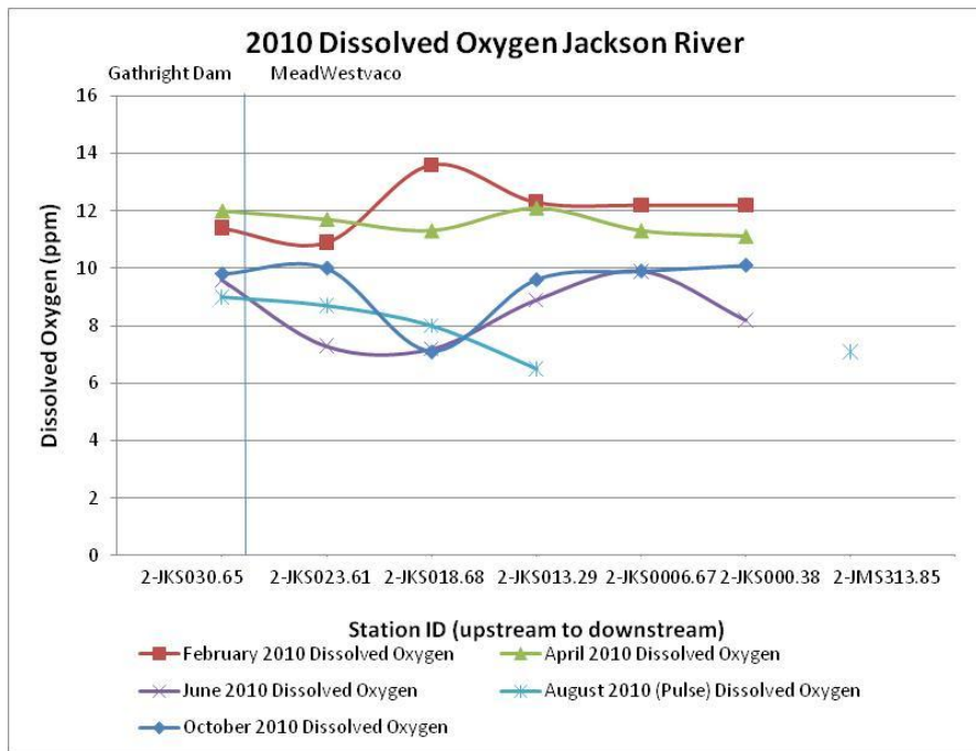
Figure 4. Dissolved oxygen (mg/L) 2010.
