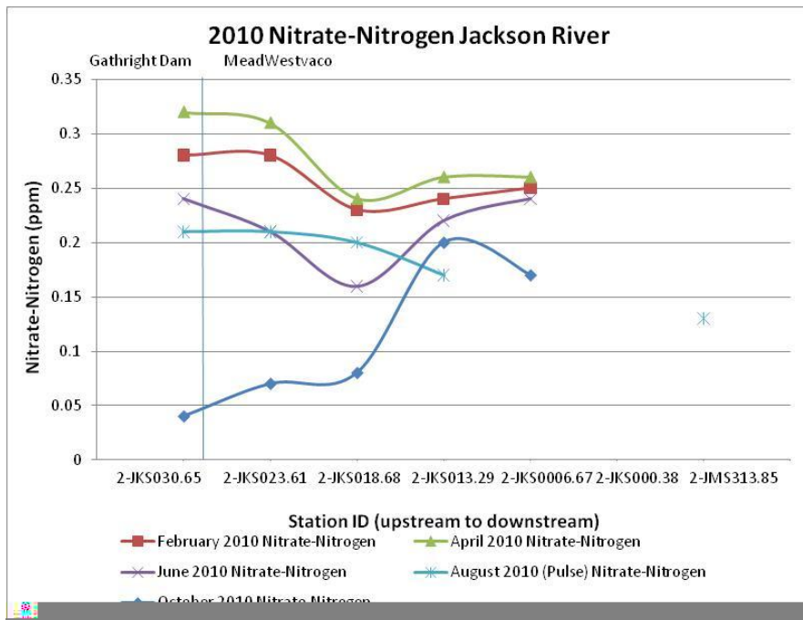
Figure 23. Nitrate-Nitrogen (mg/L) 2010.
