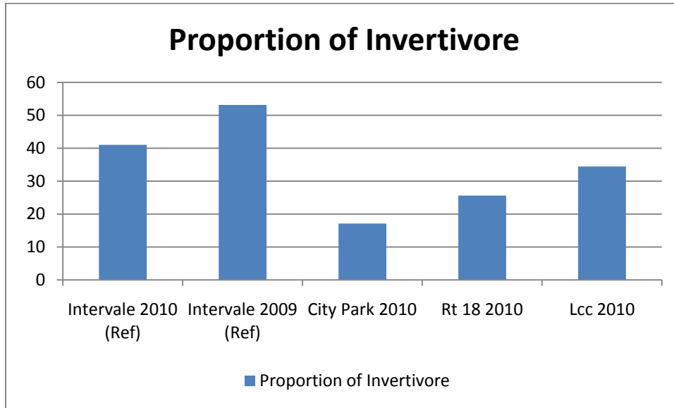
Figure 56. Proportion of invertebrates collected at each Jackson River sampling site.
