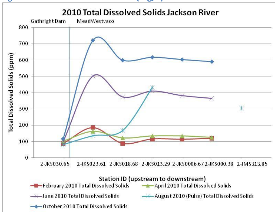
Figure 19. Total Dissolved Solids (mg/L) 2010.
